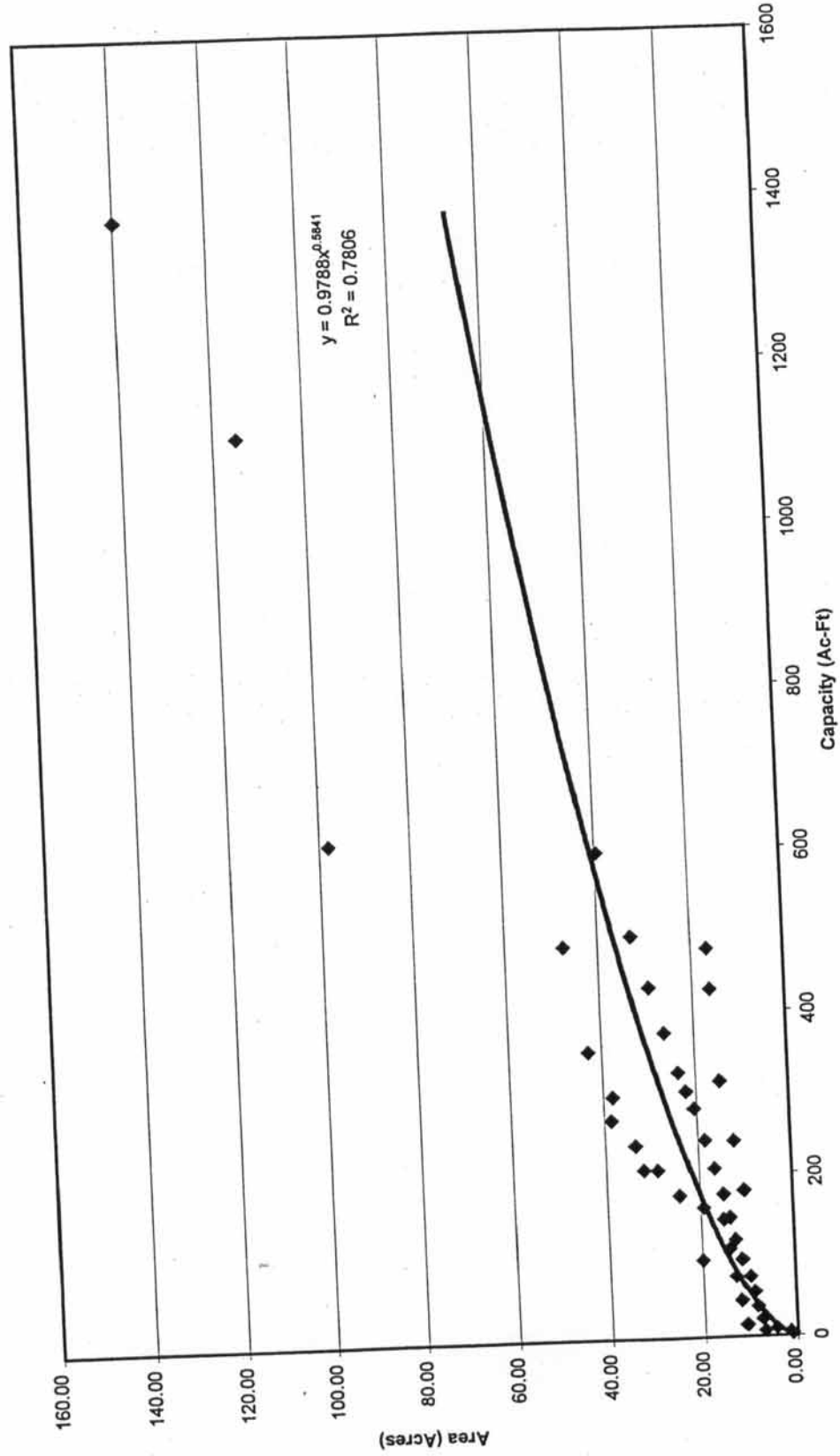
Figure 11 Cypress Basin Standard Area-Capacity Curve Reservoirs Less Than 5,000 acre-feet
